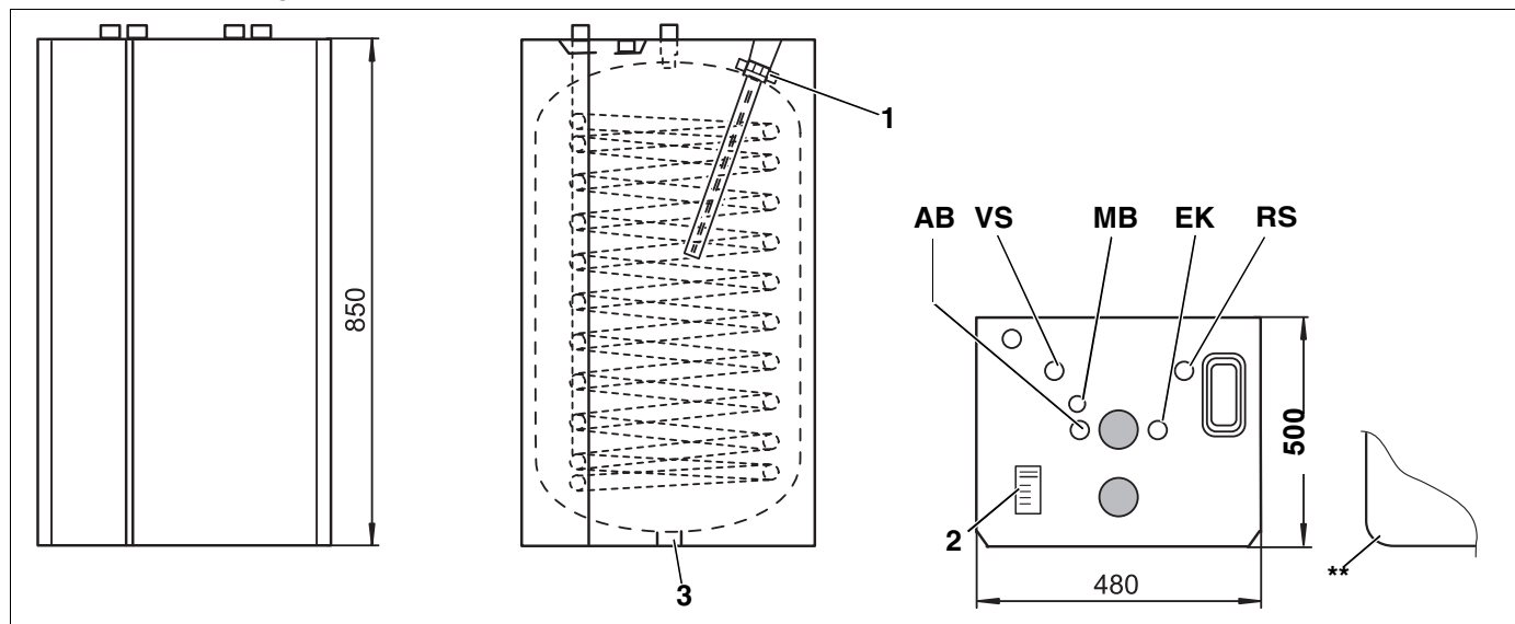
Sl. 1 Dimenzije Logalux HT 110 W/H 110 W
